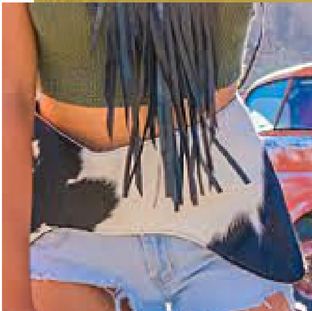
CONFIDENCE
